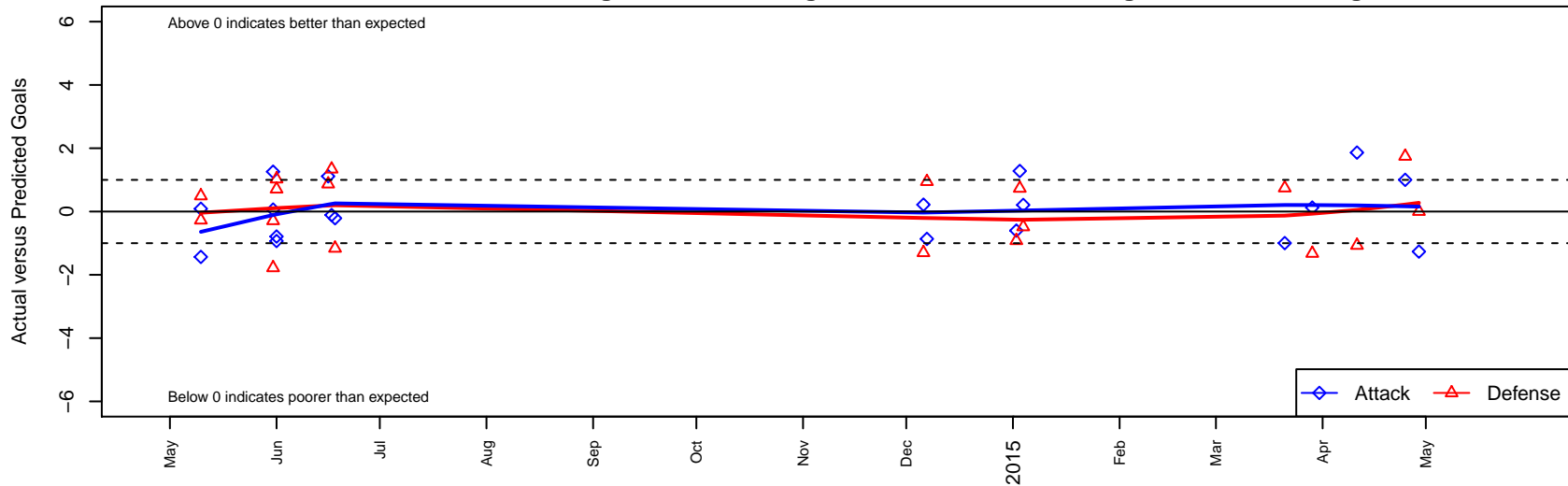
Sting SC B97 Dots are actual minus expected GF (blue circles) and GA (red triangles). Blue line is smoothed change in attack strength. Red is smoothed change in defense strength.
